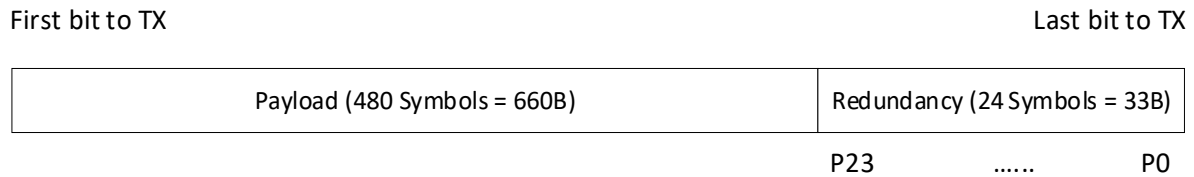
Figure 4-30. Structure of Gen 4 RS-FEC Block
