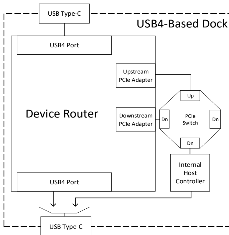
Figure 13-11. Example of a USB4-Based Dock with an Internal Host Controller
