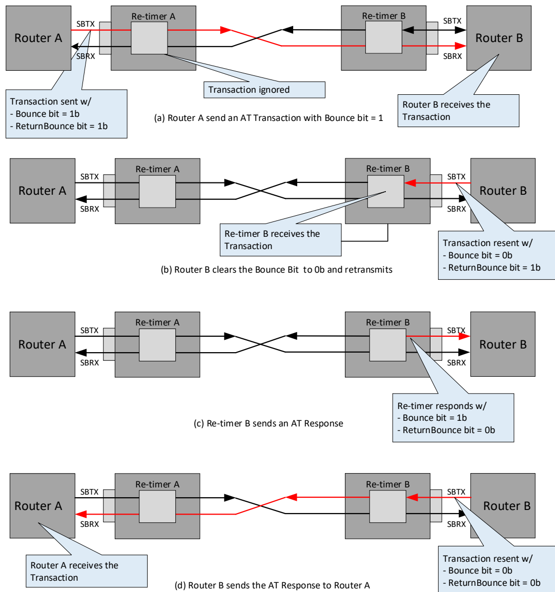
Figure 13-2. Bounce Mechanism
