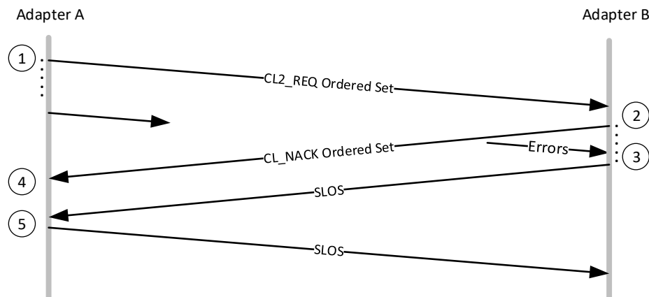
Figure C-7. Errors in CL2_REQ Reception and CL_NACK Response
