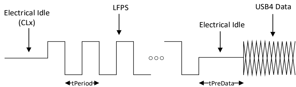
Figure 3-43. Signaling During Power Management State Exit
