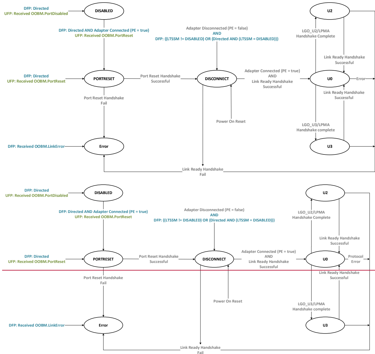
Figure 9-19. USB3 Gen T LTSSM
