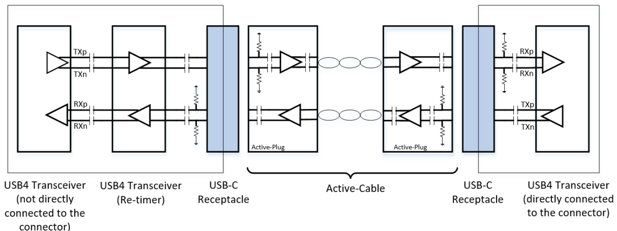
Figure 3-26. Example AC-Coupling Capacitors Placement
