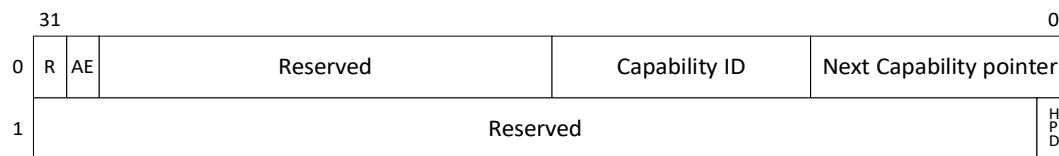
Figure 8-15. Structure of DP OUT AUX Adapter Configuration Capability
