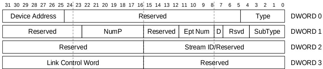
Figure 9-29. ERDY Transaction Packet
