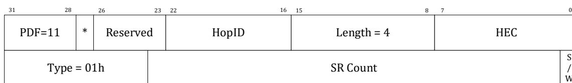
Figure 10-63: ALPM DP Link Control Packet Format
