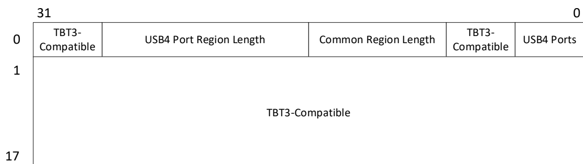
Figure 13-7. Structure of the Common Region
