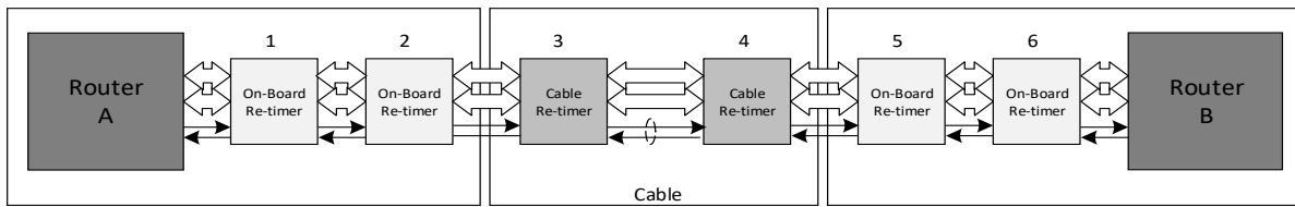
Figure 4-8. Progression of Link Equalization
