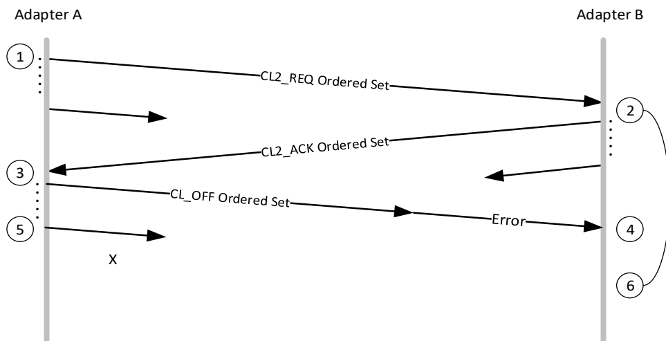
Figure C-9. Error in CL_OFF Ordered Sets
