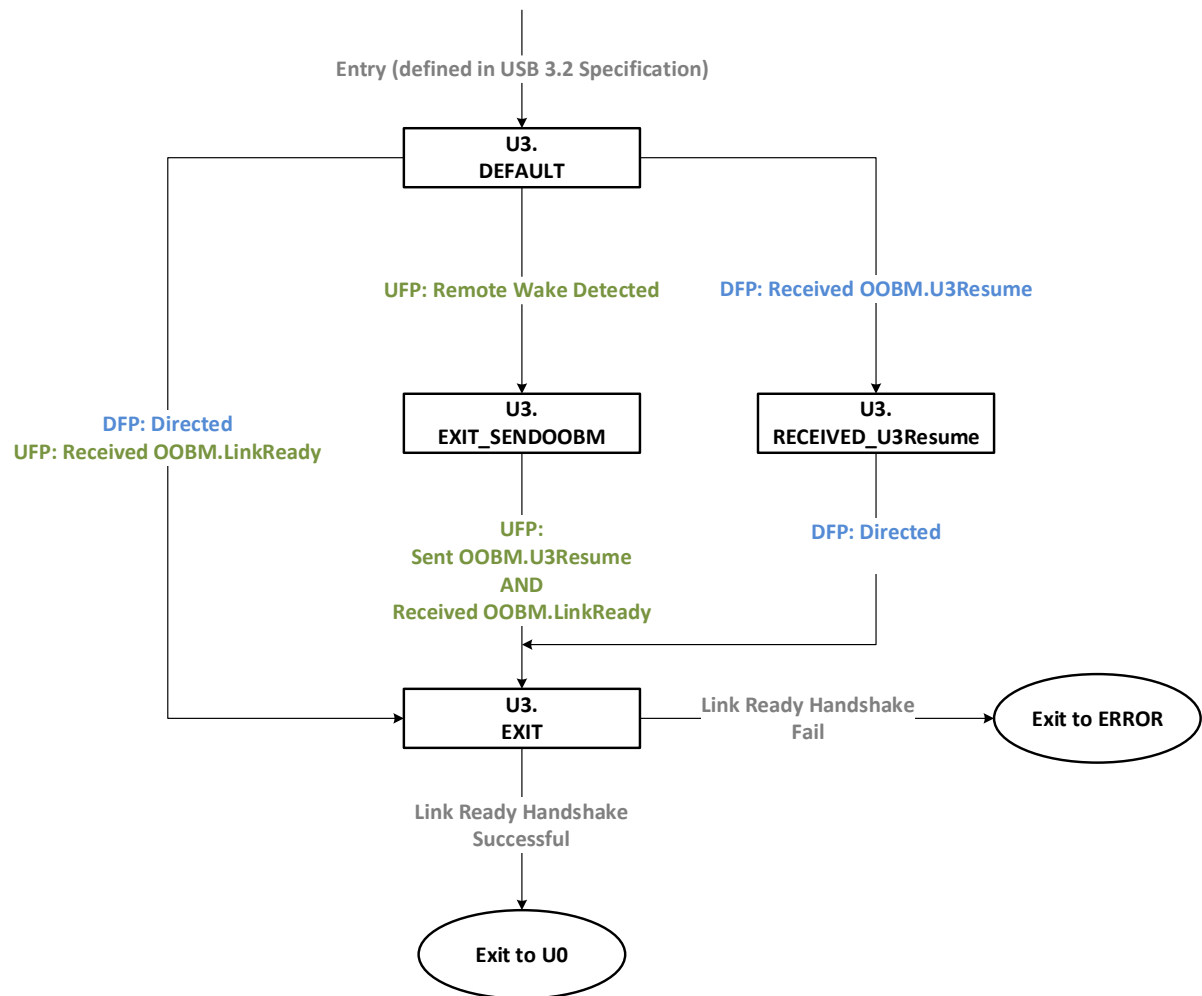
Figure 9-22. Example U3 Substate Machine
